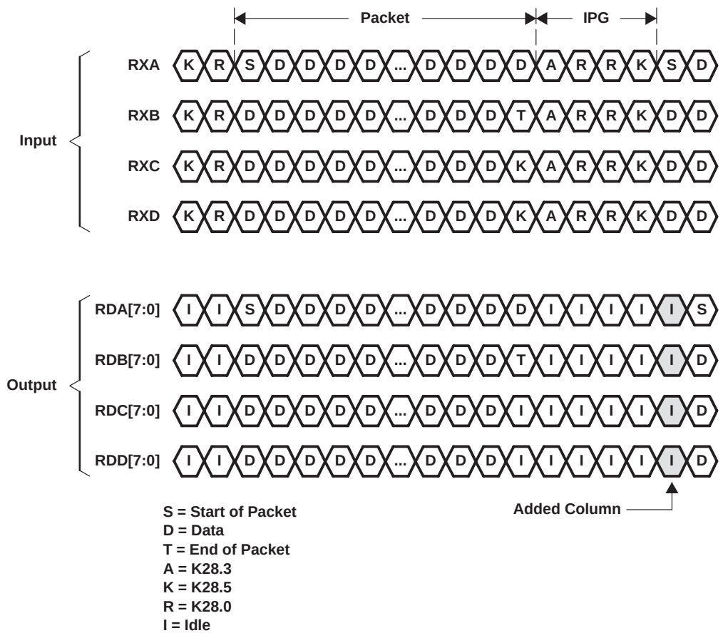
Figure 3–15. Clock Tolerance Compensation: Add
